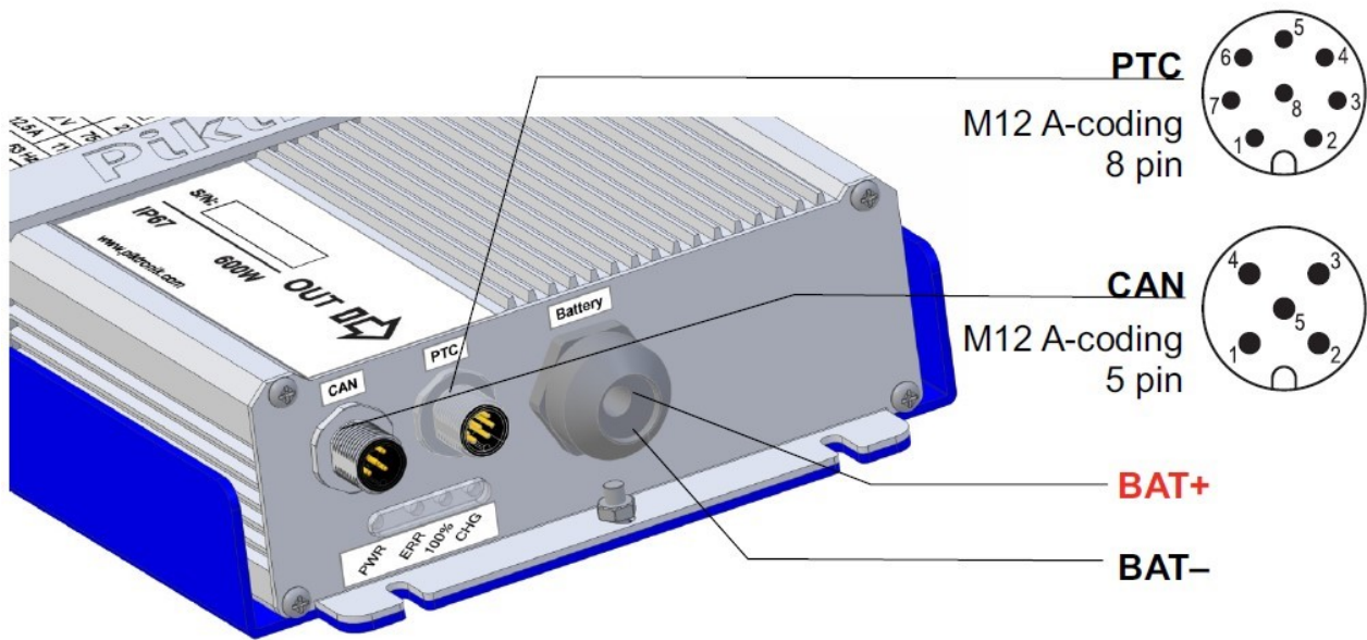
All contact arrangements shown from the mating side.
